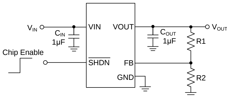
Figure 3. UM1750S-00/UM1750Y-00/UM1750DA-00 (Adjustable V OUT ) Typical Application Circuit
